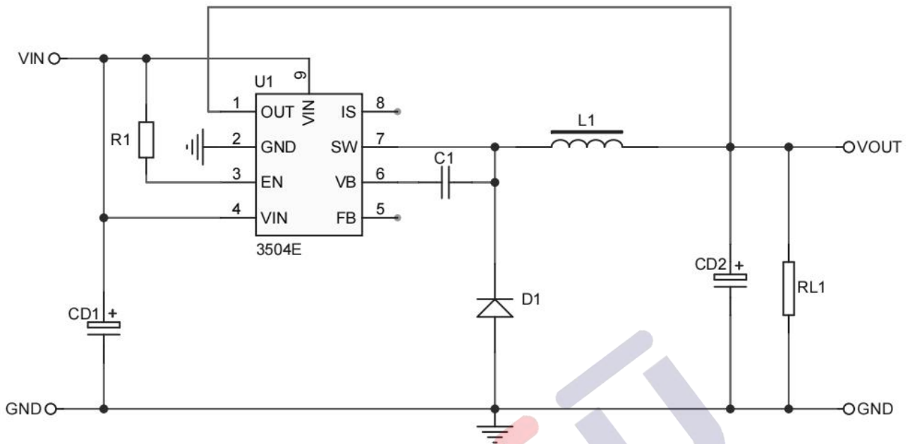
APP1: V_{OUT} = 5V
